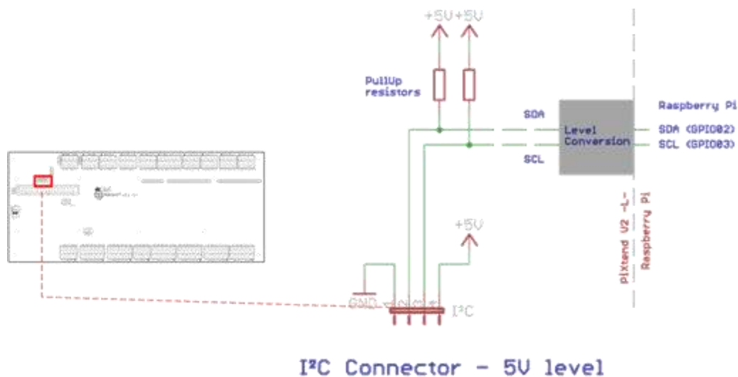
Figure 48: Simplified wiring diagram: I²C at 5V level
