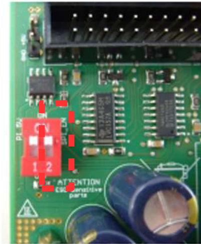
Figure 51: DIP switch: SPI_EN
