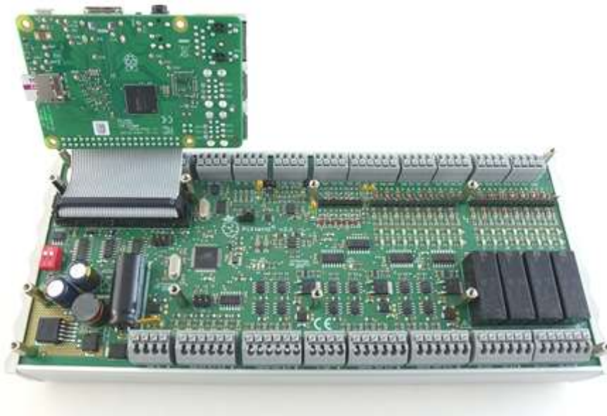
Figure 19: Raspberry Pi unscrewed from the PiXtend (ribbon cable remains connected)
