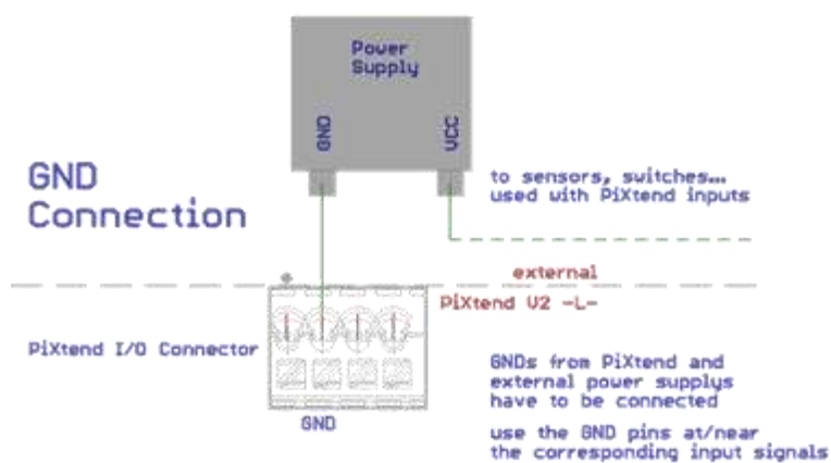
Figure 73: Simplified wiring diagram: GND connection
